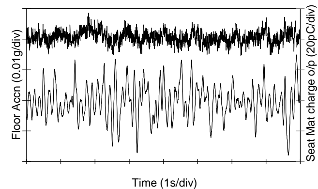
Figure 6: Cable mat installed in passenger seat of an automobile (lower trace), showing high amplitude, low frequency signals compared with chassis acceleration (upper trace)
