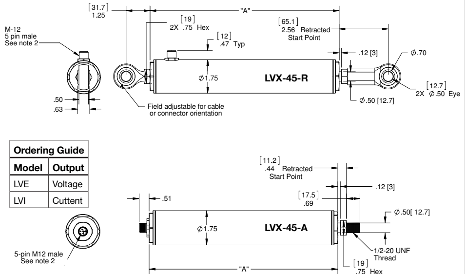
Radial Connector with Rod Eye End
