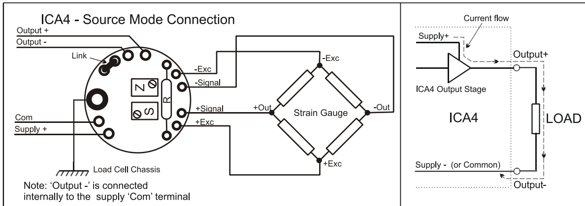
Figure 2.2 Connection Details for the ICA4 - Source mode
