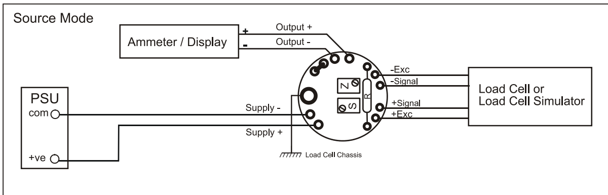
Figure 4.1 Connection Details for Calibration
