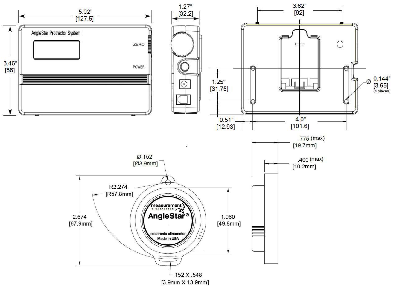
Dimensions are in inches [mm], and are nominal unless otherwise specified
