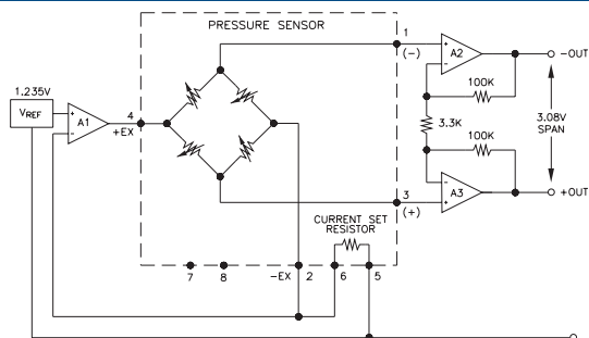
FIGURE 1: CURRENT SET CIRCUIT
